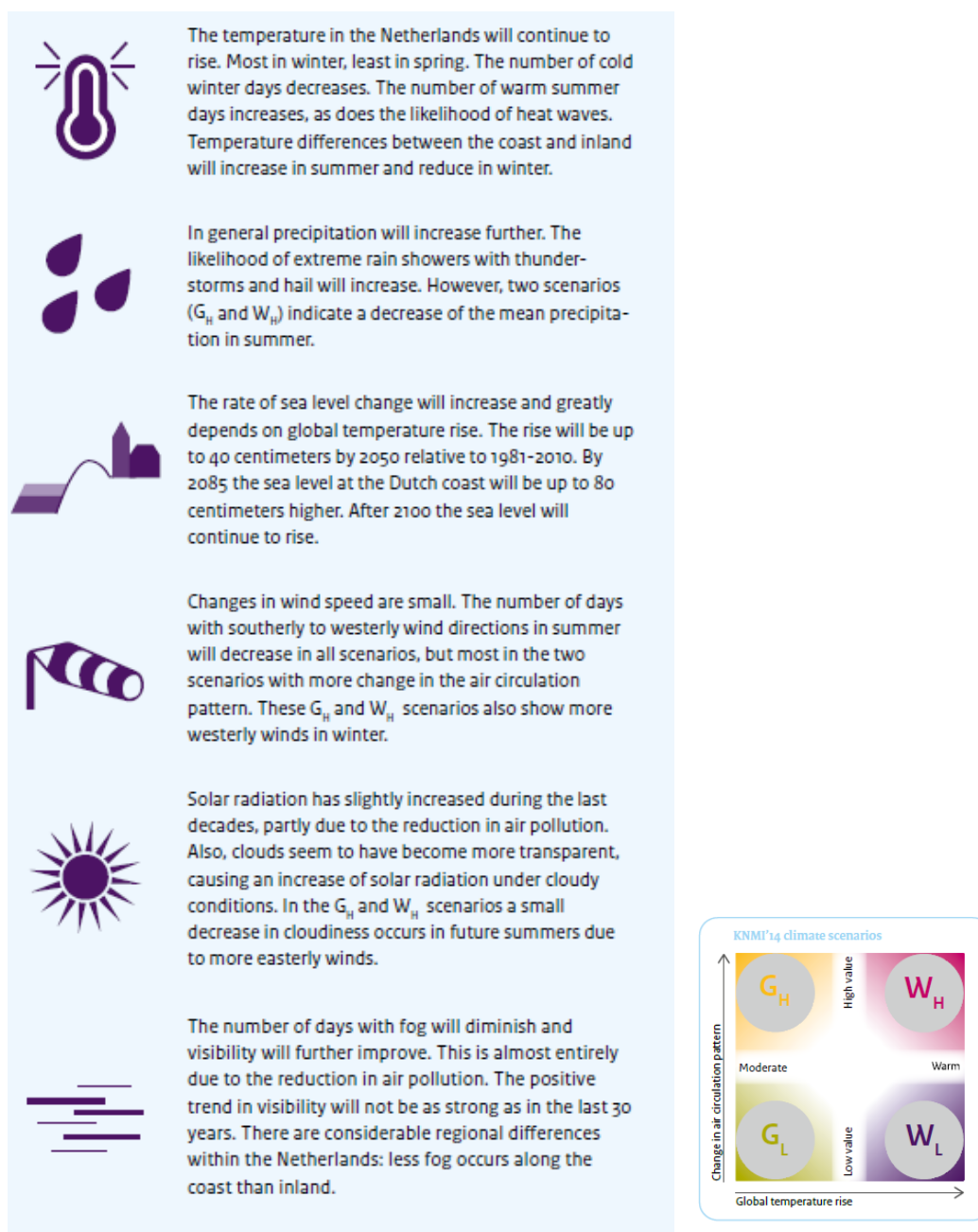
Figure 4: Projected changes in the weather because of climate change in the Netherlands
